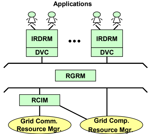
Figure 2. Structure of the RT DVC middleware effective form.
