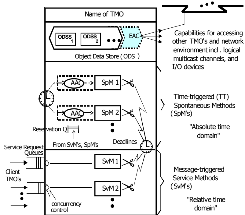
Figure 4. TMO structure
