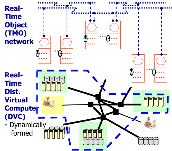
Figure 1. A real-time DVC
